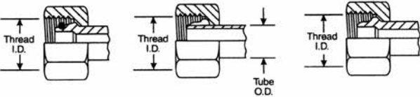
Female 24° Cone with O-Ring
