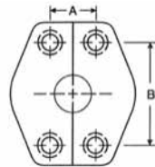
4-Bolt Split Flange
